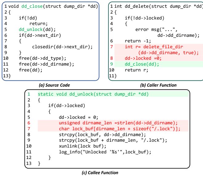
Figure 1: An inter-procedural vulnerability example of the CWE-20. Lines highlighted in green denote the call relation (i.e., callee and caller), and red denotes the vulnerable statements.
