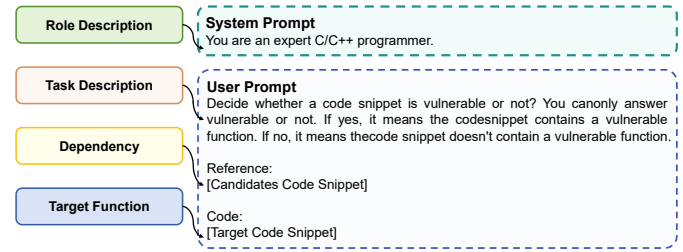
Figure 4: The Prompt Template of VulEval.
