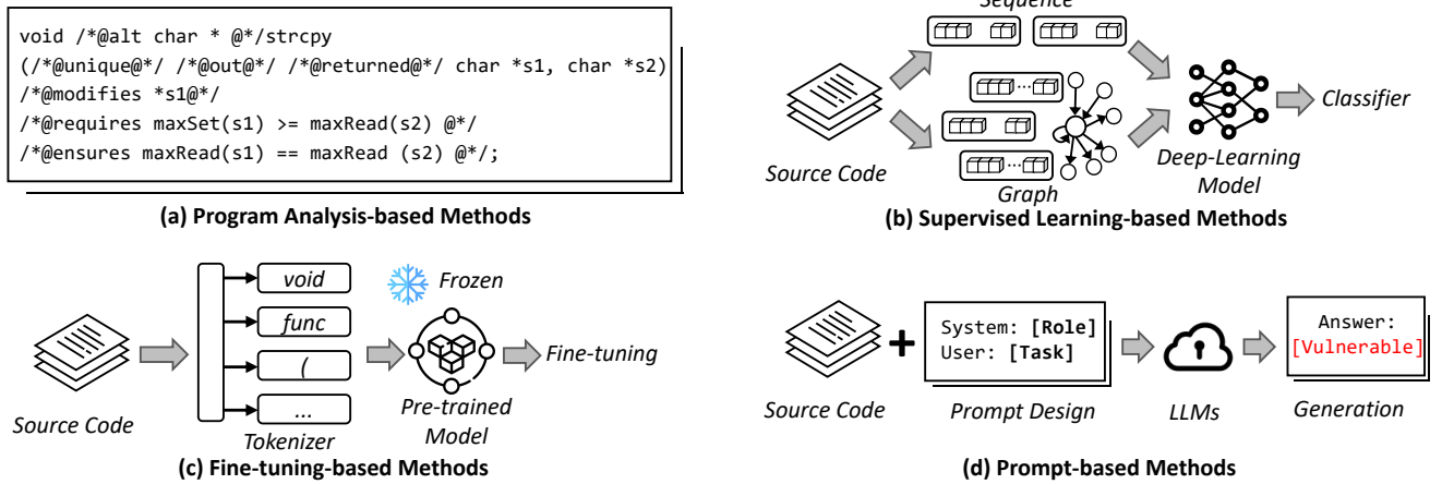
Figure 2: The four types of vulnerability detection methods.
